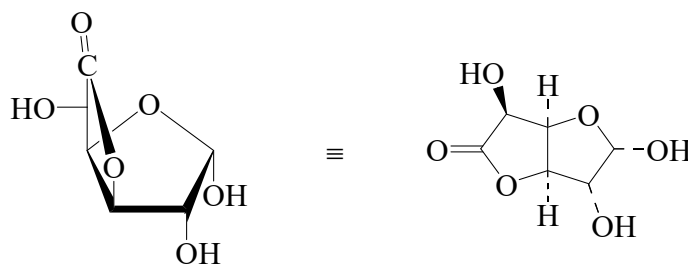
α-D-Furanose-form
